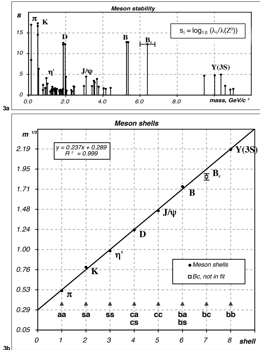
Fig. 3. Meson shells: 3a, meson stability plot, s_i = \log_{10} (\lambda_i / \lambda(Z^0)) vs mass, with evidence of meson shells 1 to 8; 3b, meson shells stability line fit with R^2 correlation parameter, and also quark composition for the various shells ( a = u \vee d ; xy = xybar \vee yxbar ).
