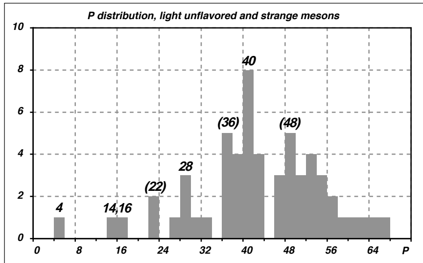
Fig. 6. Light unflavored mesons and strange mesons: 6a, meson stability vs mass as in figure 5 but on a restricted mass range, with scale in steps of 70 MeV/c 2 ; meson clusters are identified by grey block arrows; 6b, histogram of P, with the (4,14,28) meson shell sequence #2, the (4,16,40) sequence #1, and 36=40-4 and 48=40+8 as sub-shell configurations.
